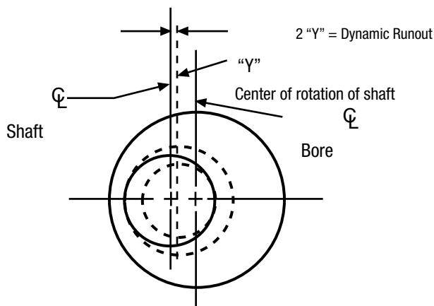
Figure 6 — Dynamic Runout
