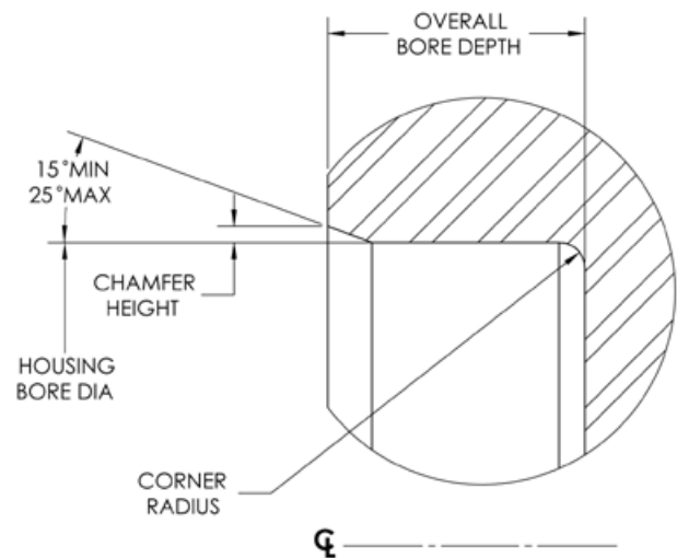
Figure 13 — Housing Bore Dimensions
