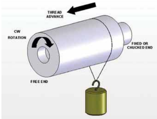
Figure 1 — Clockwise Lead
