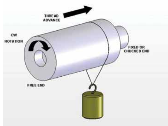
Figure 4 — Counter-Clockwise Lead
