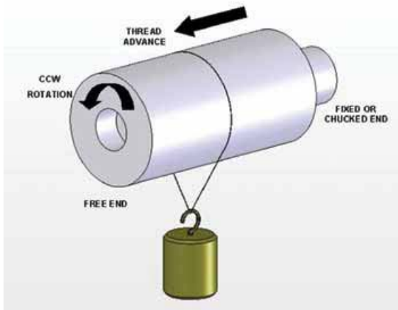
Figure 3 — Counter-Clockwise Lead
